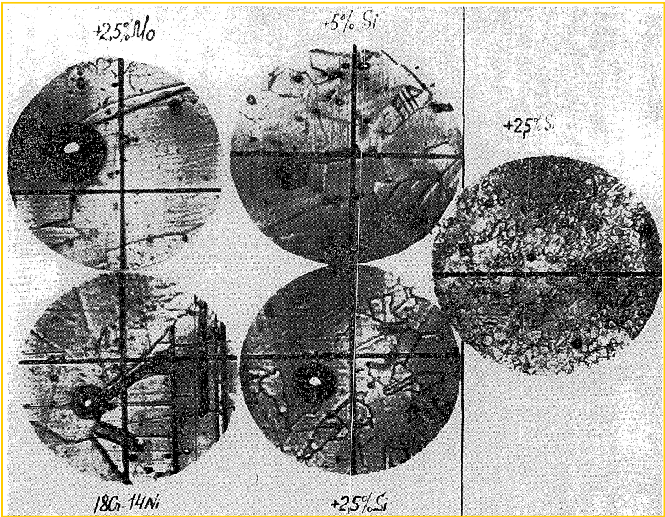
Figure 5—Site of pitting initiation on 18Cr-14Ni steels additionally alloyed with Mo and Si. The perpendicular lines on the photograph represent the cross-hairs of the microscope eyepiece. 700X except photo at extreme right, which is 200X
